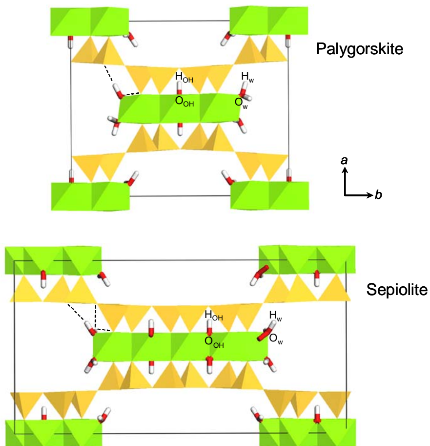
Figure 1.1 Polyhedra models of the unit cells of palygorskite (top) and sepiolite (bottom) derived from VASP DFT optimizations. Yellow tetrahedra and green octahedra represent coordinated Si and Mg atoms, respectively. Structural water molecules and hydroxides are highlighted as cylinders (O is red, H is white). Abbreviations O_{OH} and H_{OH} refer to hydroxyl oxygen and hydrogen, while O_w and H_w refer to water oxygen and hydrogen. All other framework oxygen atoms are abbreviated O_F in the text. Selected hydrogen bonds associated with structural water are shown as dashed lines.
