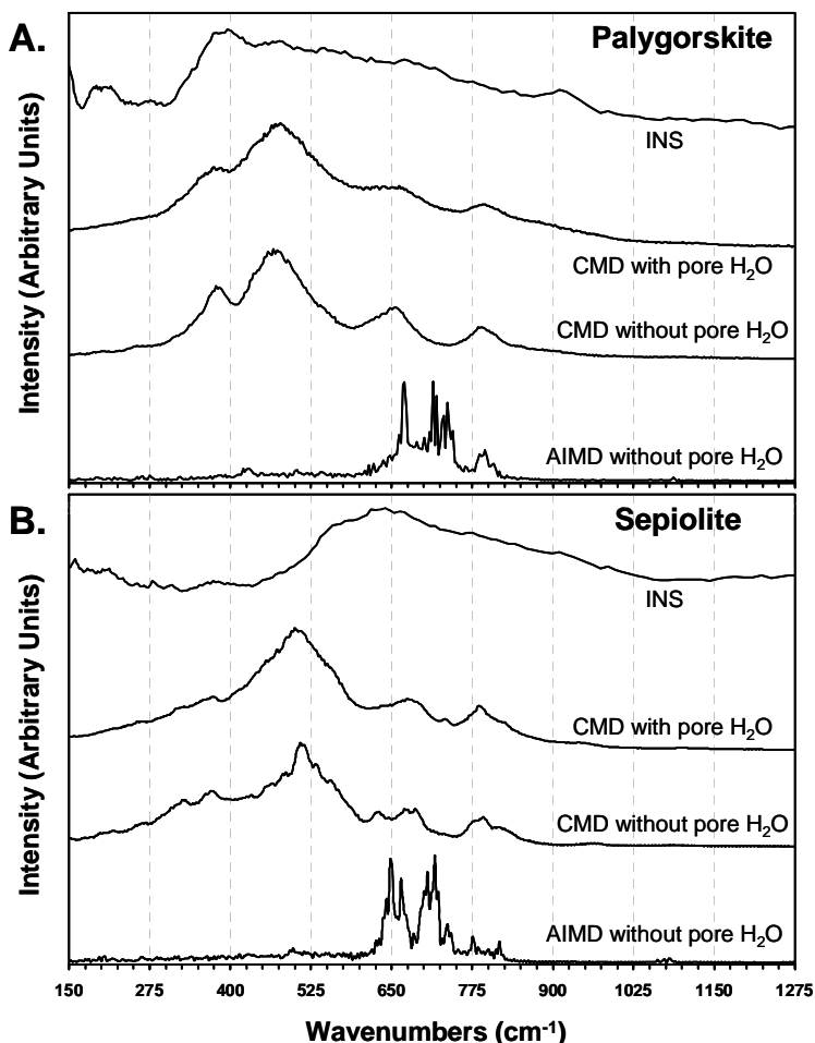
Figure 4.1 Comparison of experimental and simulated librational spectra of the hydrogen-containing components of (A) palygorskite and (B) sepiolite. All spectra correspond to 90 K except AIMD, which corresponds to 300K.
