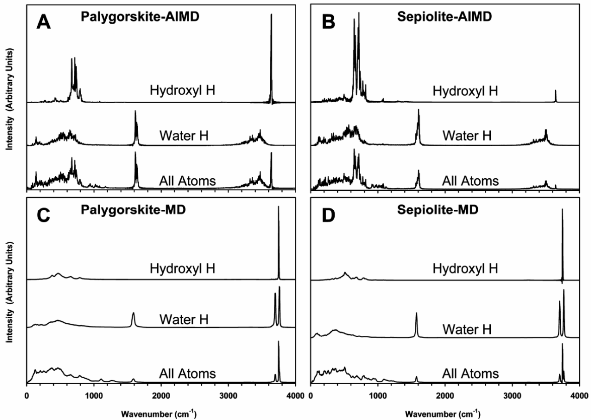
Figure 3.2 Hydroxyl H, water H, and all-atom (without pore waters) power spectra at 300 K of (A) AIMD palygorskite and (B) AIMD sepiolite and (C) CMD palygorskite and (D) CMD sepiolite.
