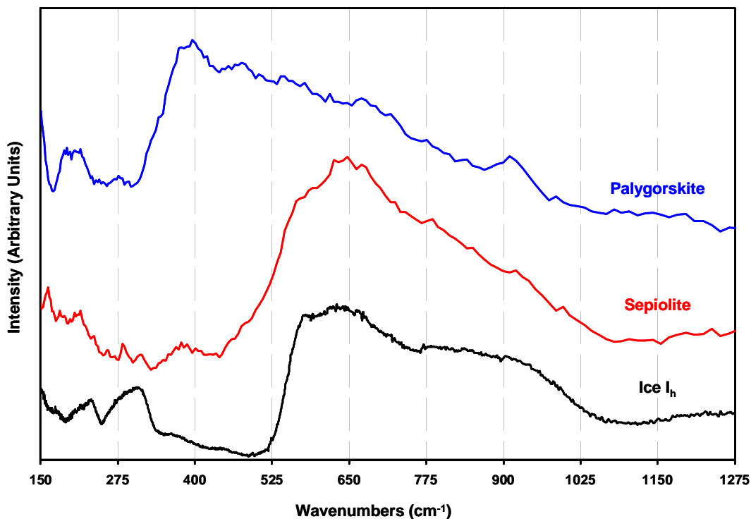
Figure 3.1 Inelastic neutron scattering (INS) data of fully hydrated palygorskite (blue), sepiolite (red), and ice I_h (black) 44,45,58 at 90 K.
