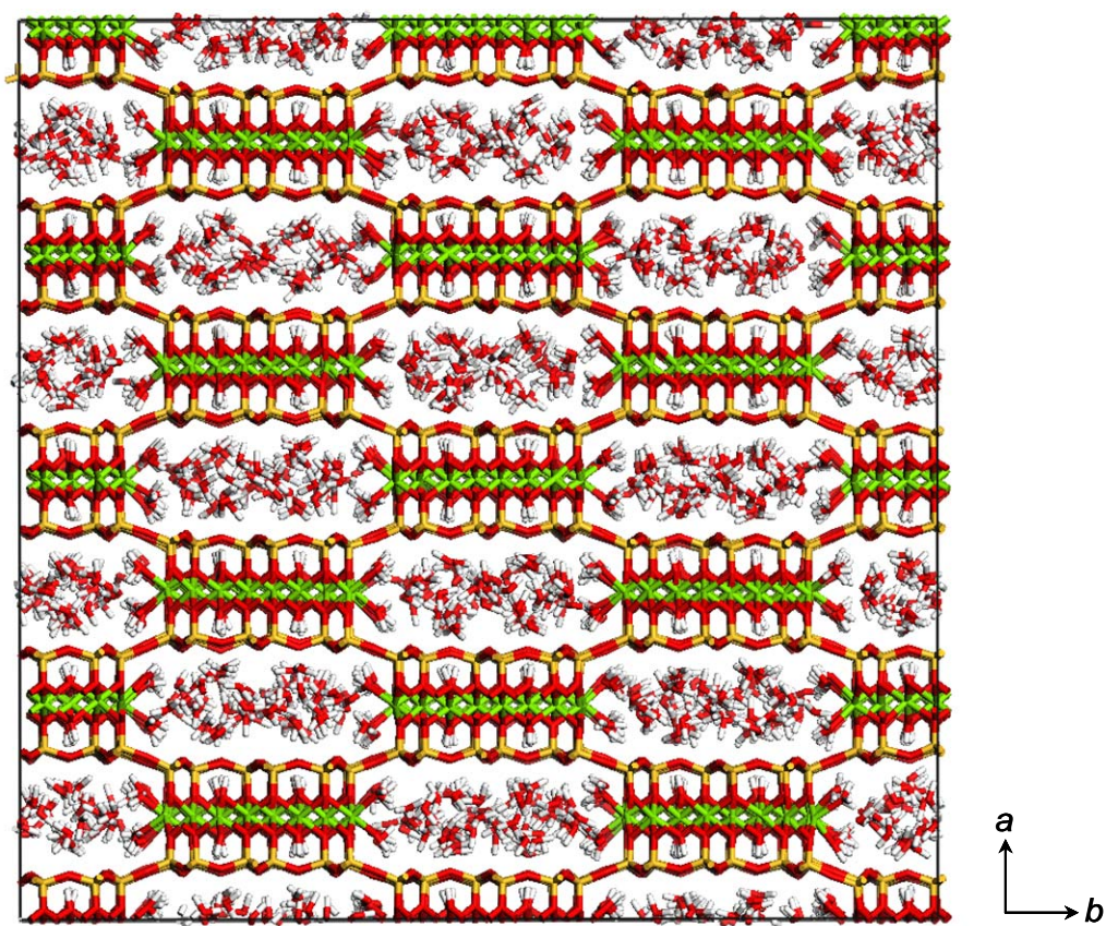
Figure 2.1 Snapshot image of the fully hydrated sepiolite structure obtained from the equilibrated trajectory associated with the CMD simulation. Water molecules occur in the sepiolite channels and coordinated to the edges of the magnesium sheets. Hydroxyls are disposed normal to the magnesium sheets. The color scheme is the same as in Figure 1.1. An equivalent simulation cell was used for palygorskite.
