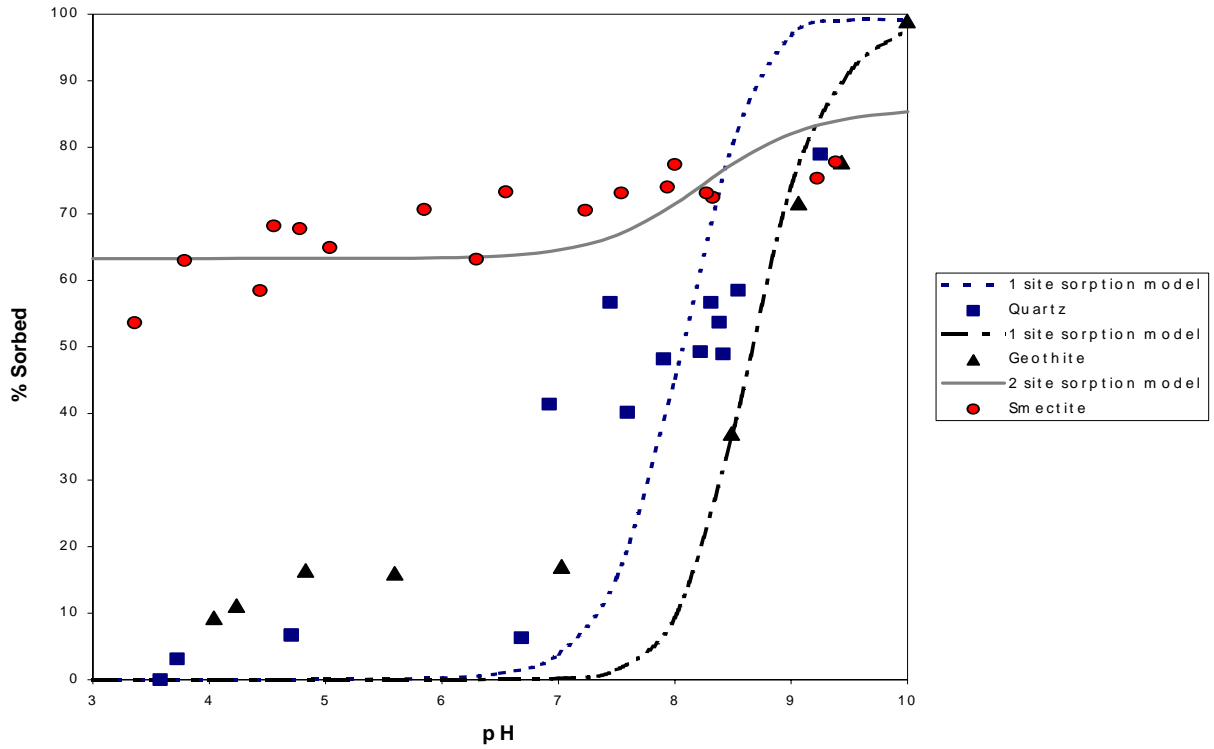
Figure 1. Effects of pH on \text{Sr}^{2+} sorption onto montmorillonite, goethite and quartz mixture.
