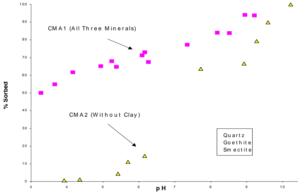
Figure 2. Effect of pH on \text{Sr}^{2+} sorption on composite mineral mixture
